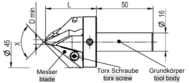
GH-K 45
