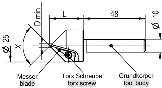
GH-K 25
