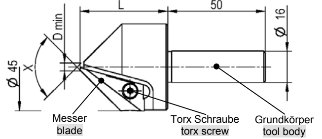
GH-K 45
